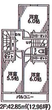
2F:42.85㎡(12.96坪)
